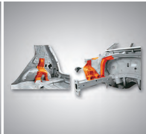
Front Fender & Rear Qtr Reinforcements for improved NVH and body rigidity for better ride and handling
