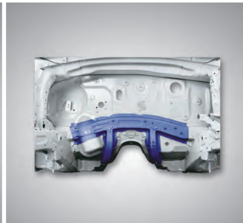
Dash Cross Members for reducing frontal crash impact
