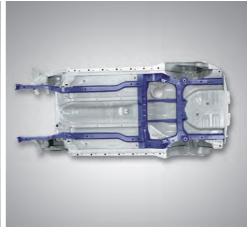
Dual Underbody Load Path for reduced frontal crash impact and improved ride and handling
