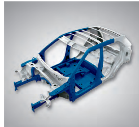
Ultra High Strength Steel Application for improved body endurance and corrosion durability. Lighter body for better mileage.
